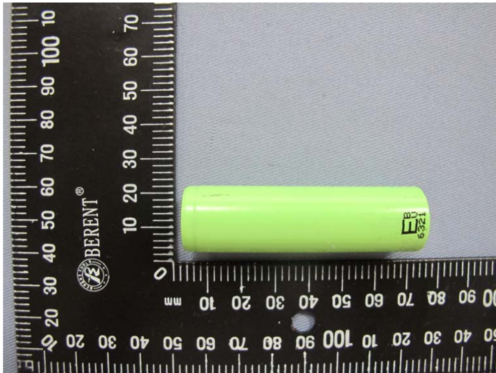
Figure 4 Bottom view of cell
